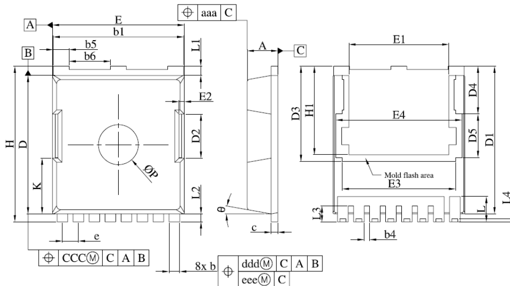
TOLL-8L Package
