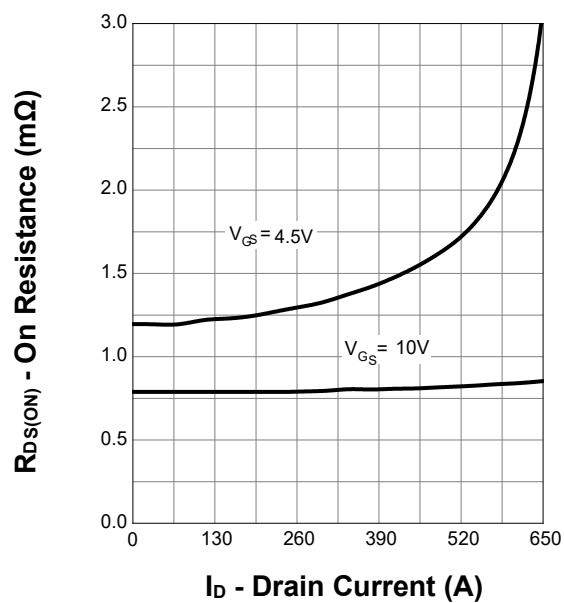
On Resistance
