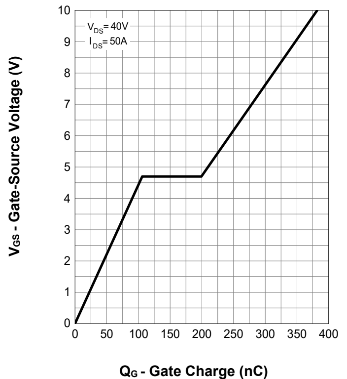
Gate Charge
