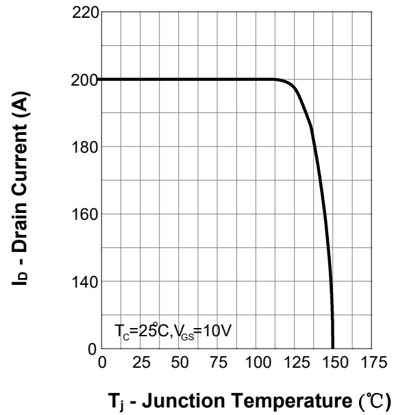
Current Capability
