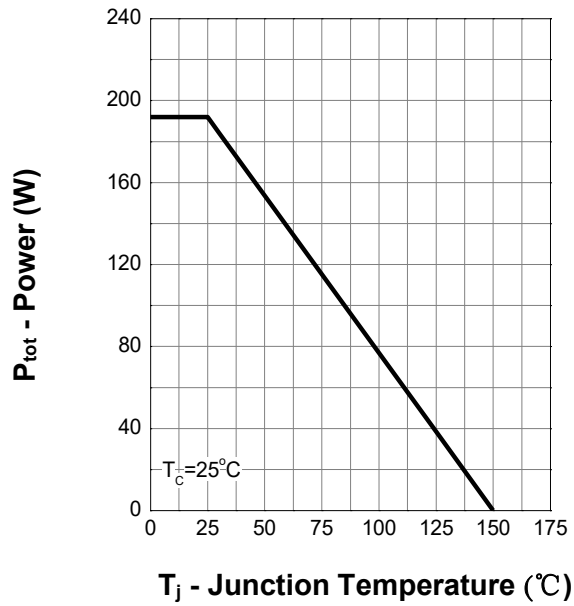
Power Capability
