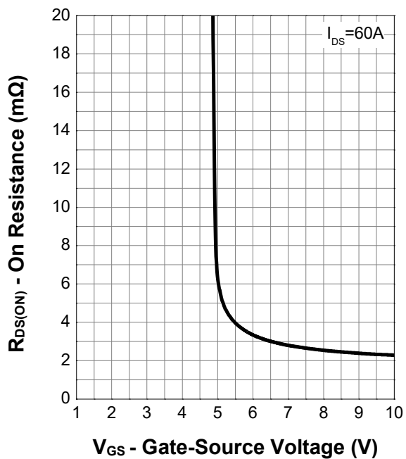
Transfer Characteristics
