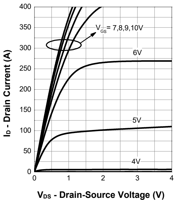
Output Characteristics
