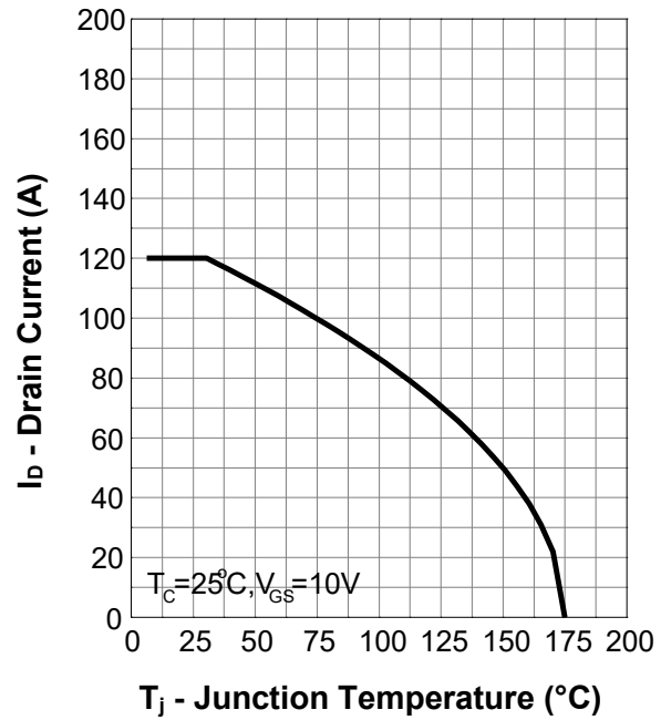
Current Capability
