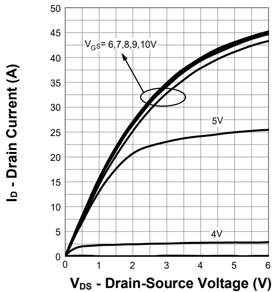
Output Characteristics
