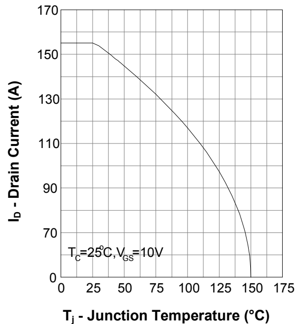
Current Capability
