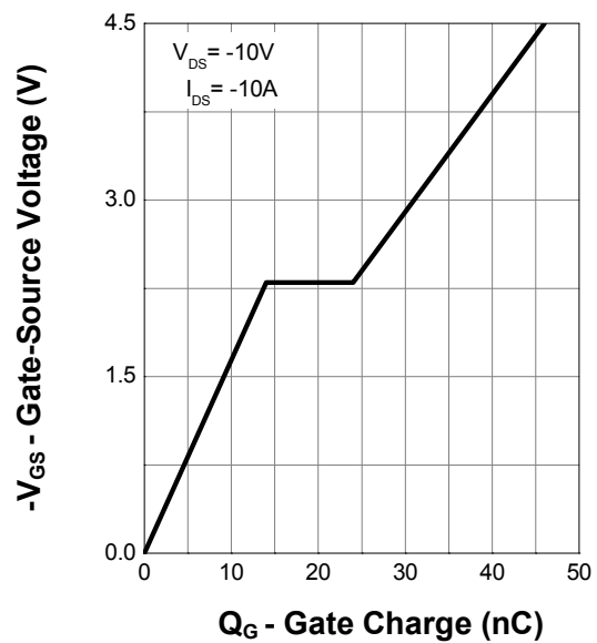
Gate Charge
