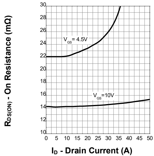
On Resistance
