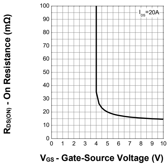
Transfer Characteristics
