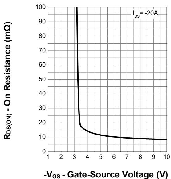
Transfer Characteristics
