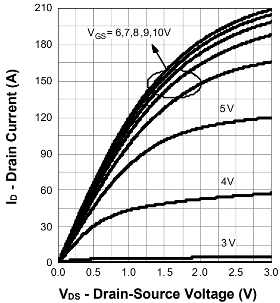
Output Characteristics
