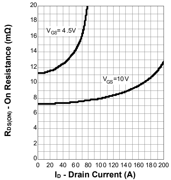
On Resistance
