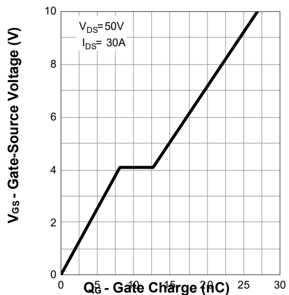
Gate Charge
