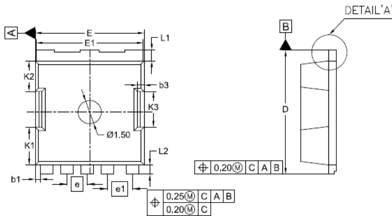
sTOLL Package
