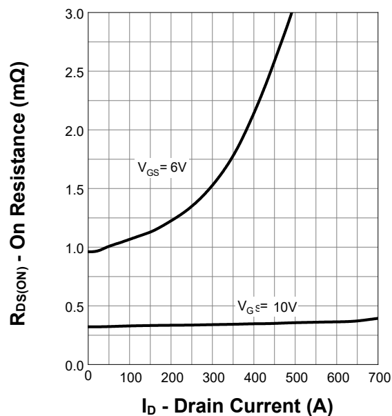
On Resistance
