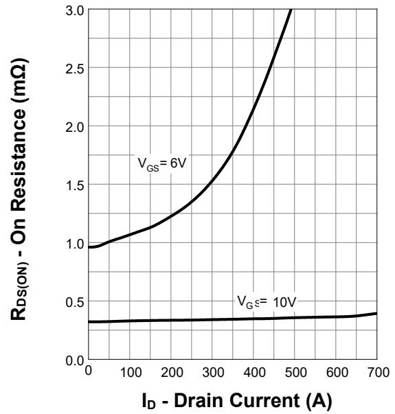
On Resistance
