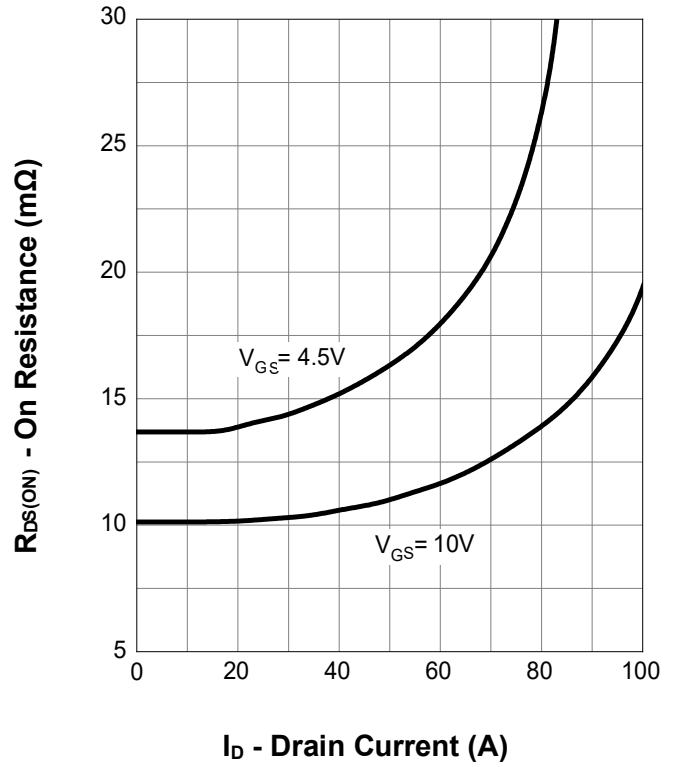
On Resistance
