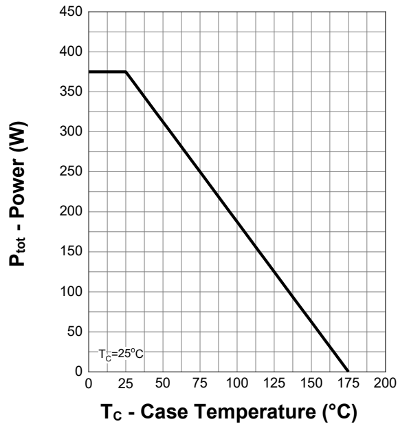
Power Capability
