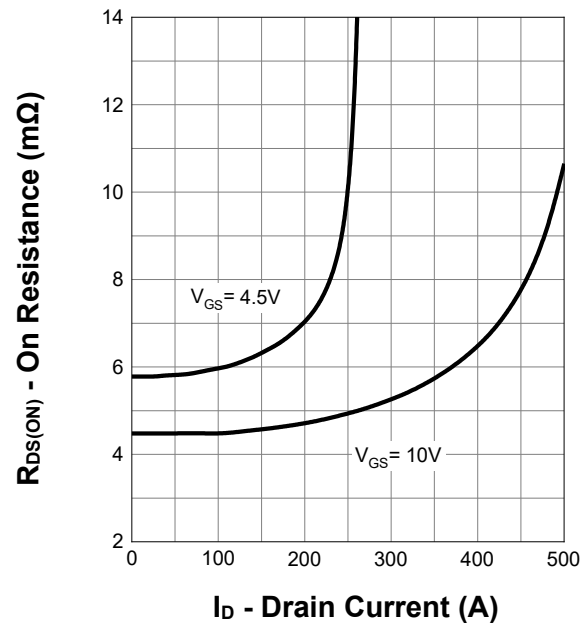
On Resistance
