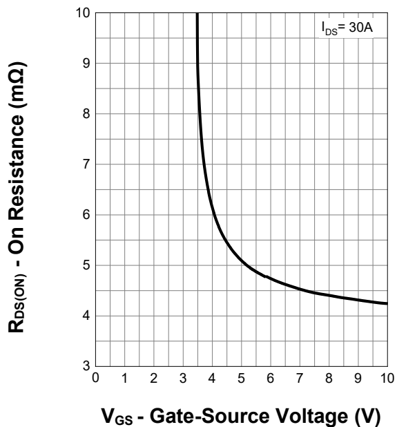
Transfer Characteristics
