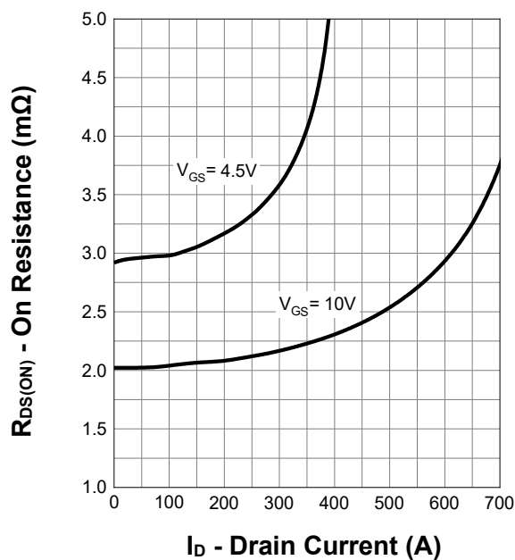
On Resistance
