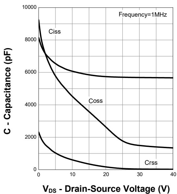
Capacitance
