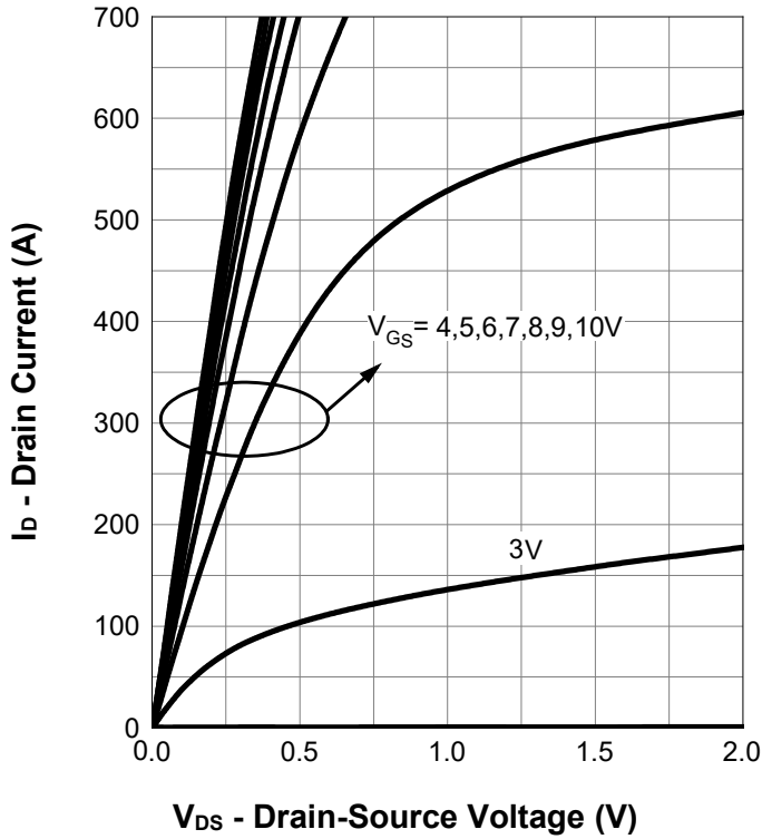
Output Characteristics
