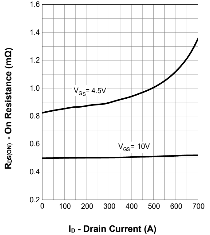
On Resistance
