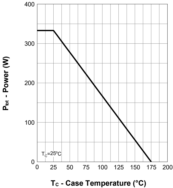
Power Capability
