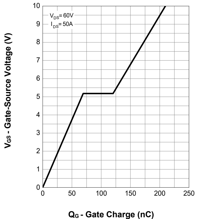
Gate Charge
