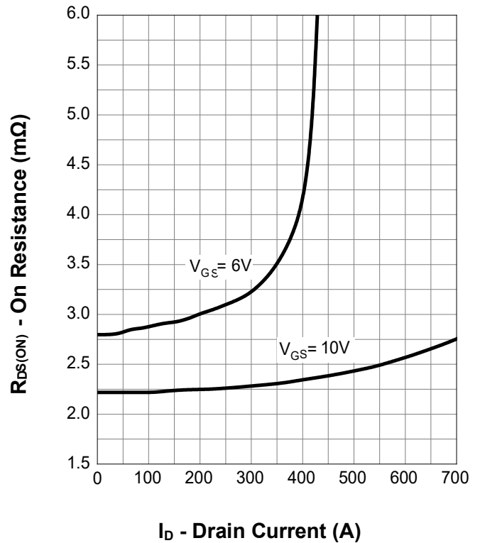
On Resistance
