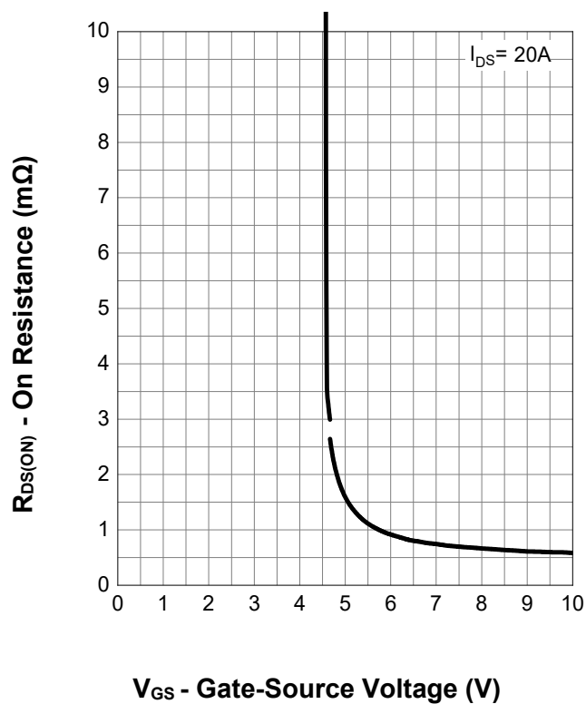
Transfer Characteristics
