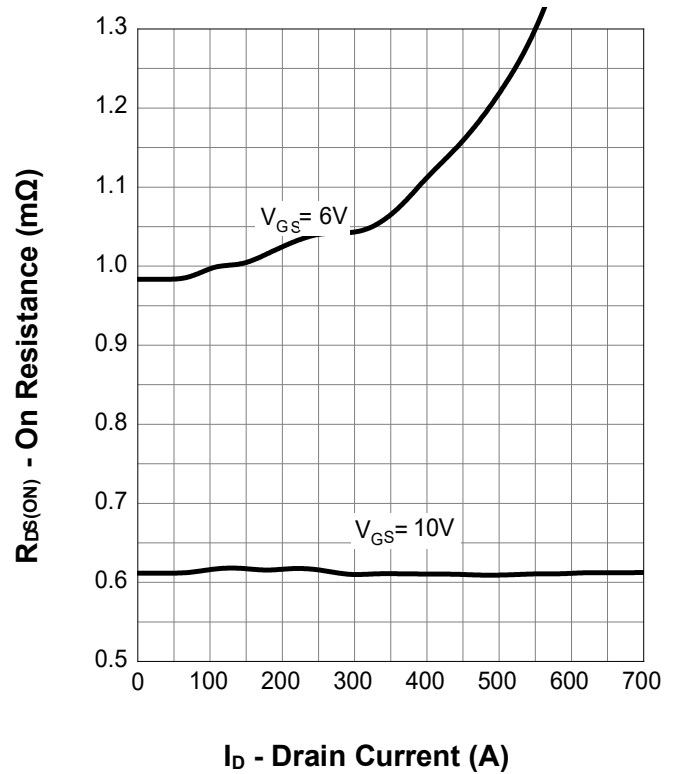
On Resistance
