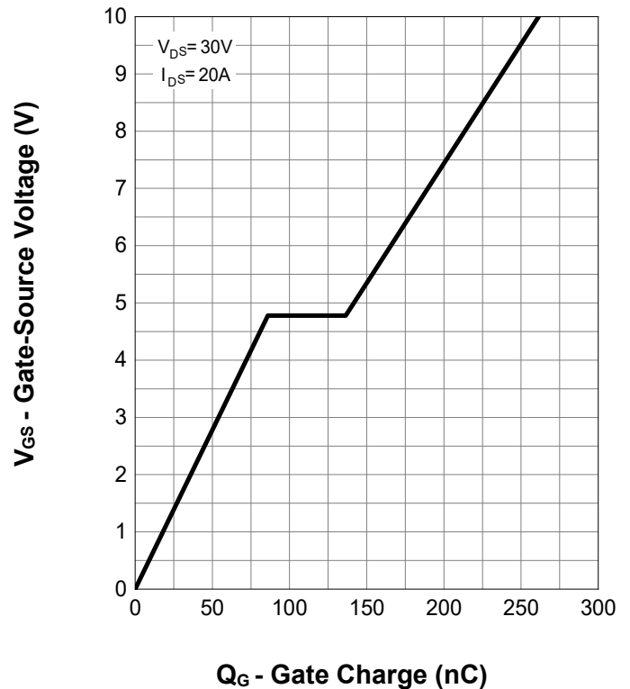
Gate Charge
