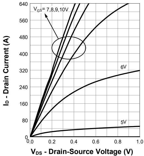
Output Characteristics
