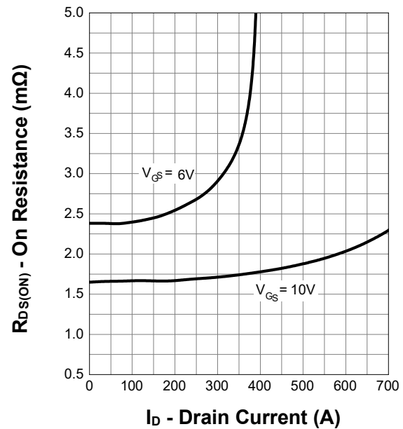
On Resistance
