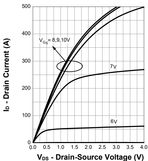
Output Characteristics
