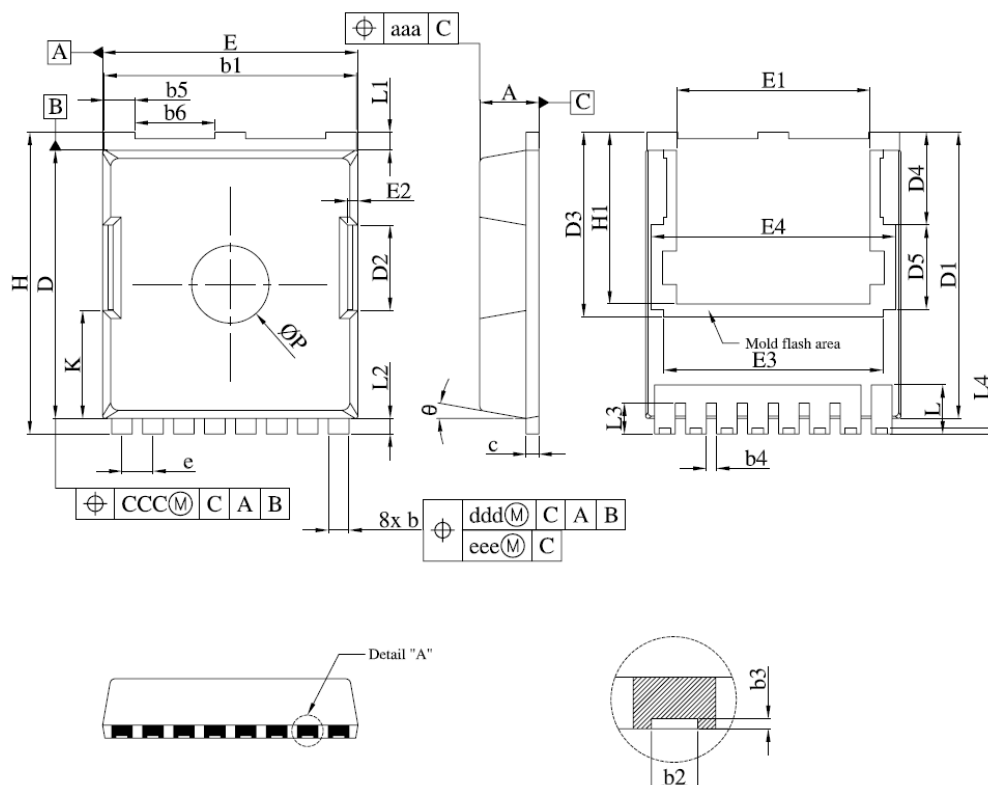
TOLL-8L Package
