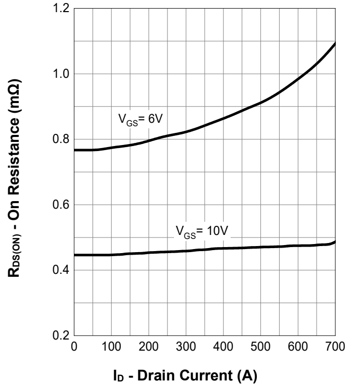
On Resistance
