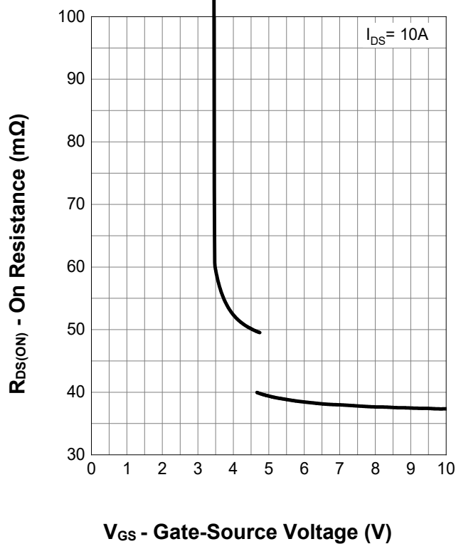
Transfer Characteristics
