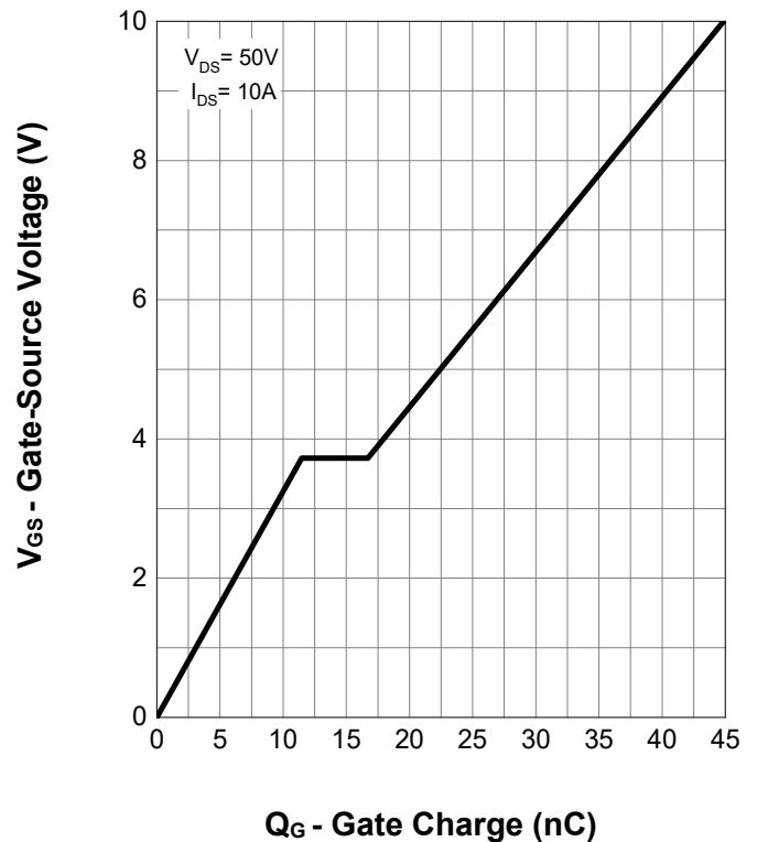
Gate Charge
