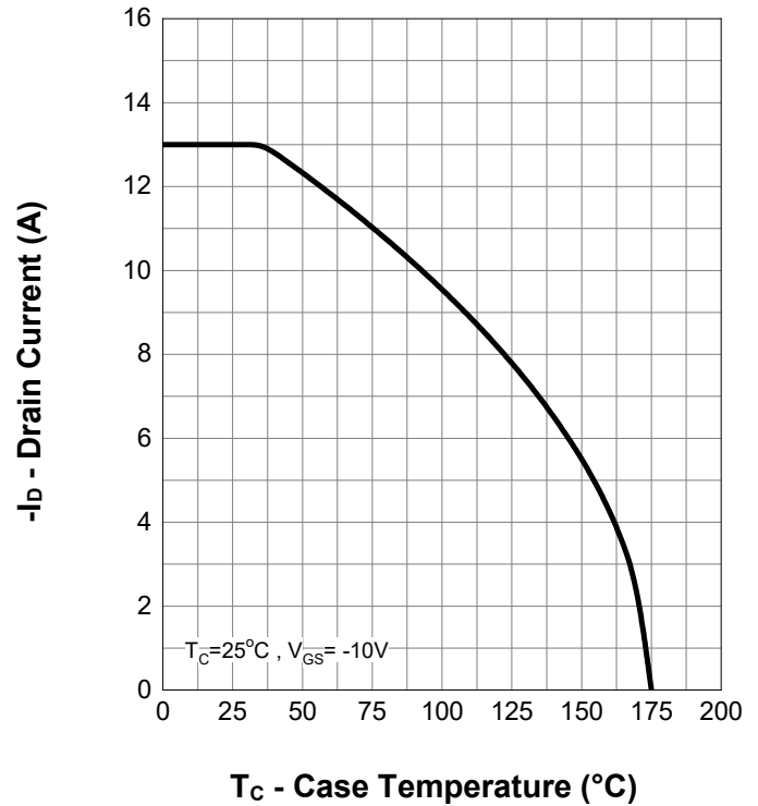
Current Capability
