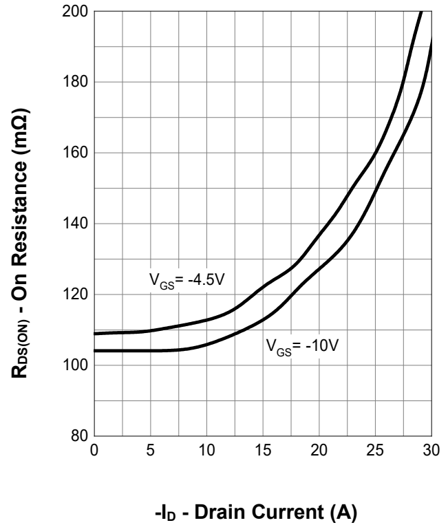
On Resistance
