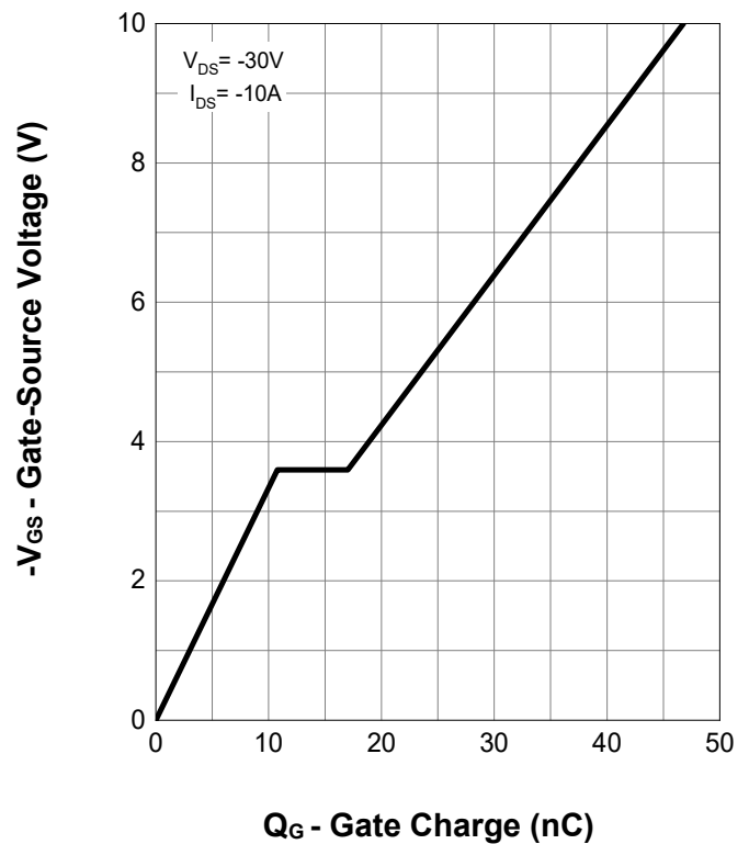
Gate Charge
