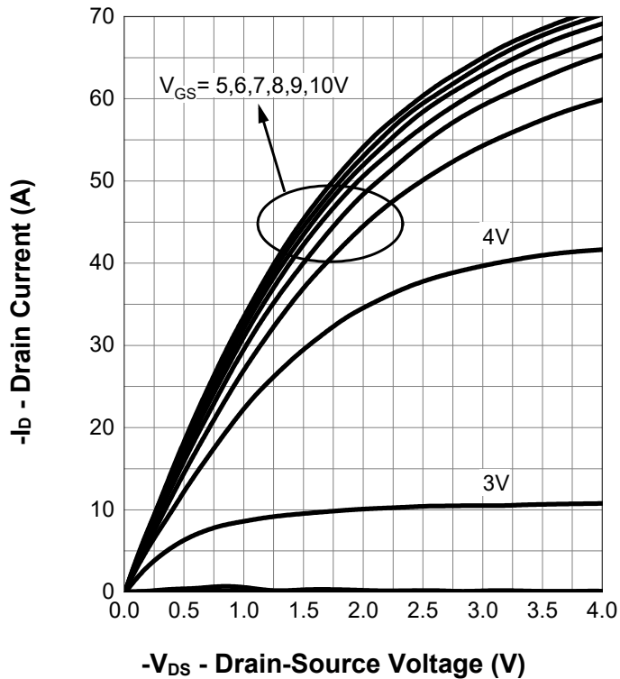
Output Characteristics
