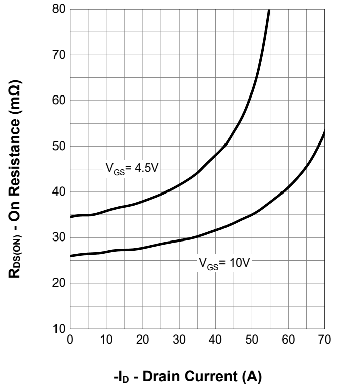
On Resistance
