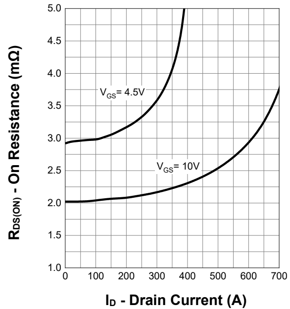
On Resistance
