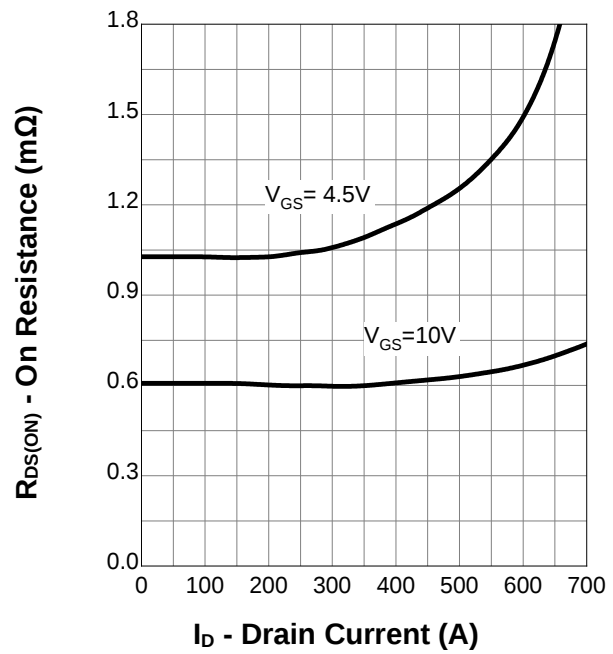
On Resistance
