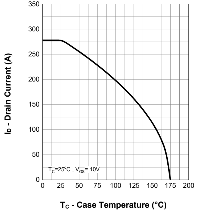
Current Capability
