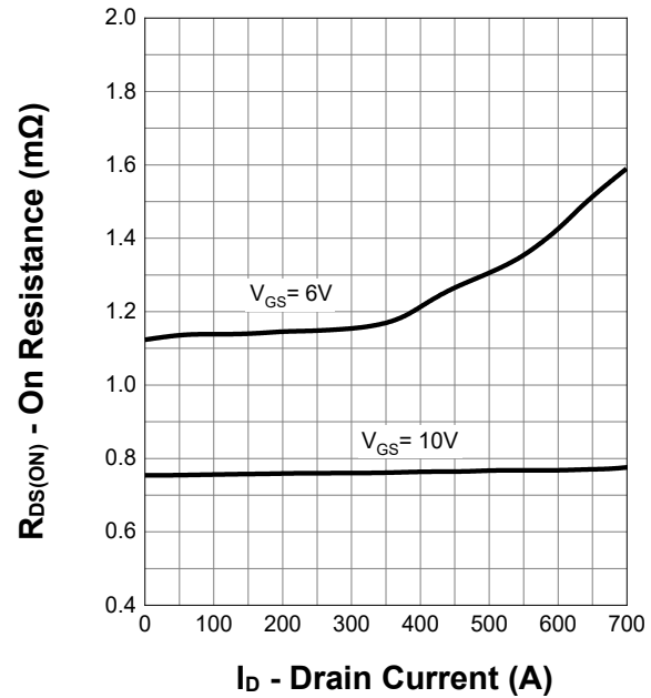
On Resistance
