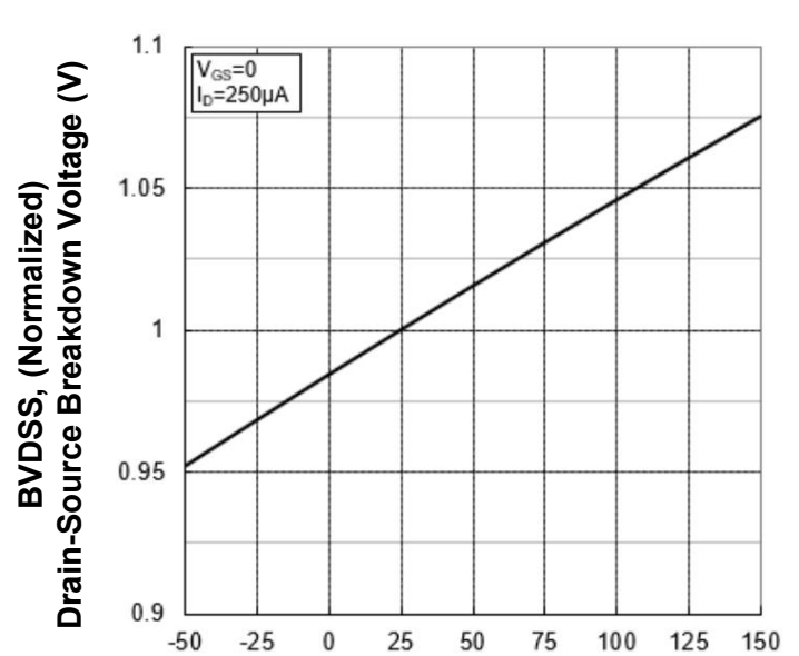
T_j - Junction Temperature ( ^{\circ}C )
