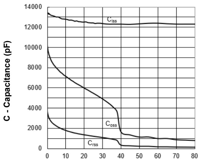
Capacitance
