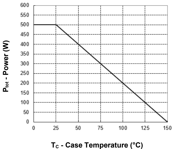
Power Capability
