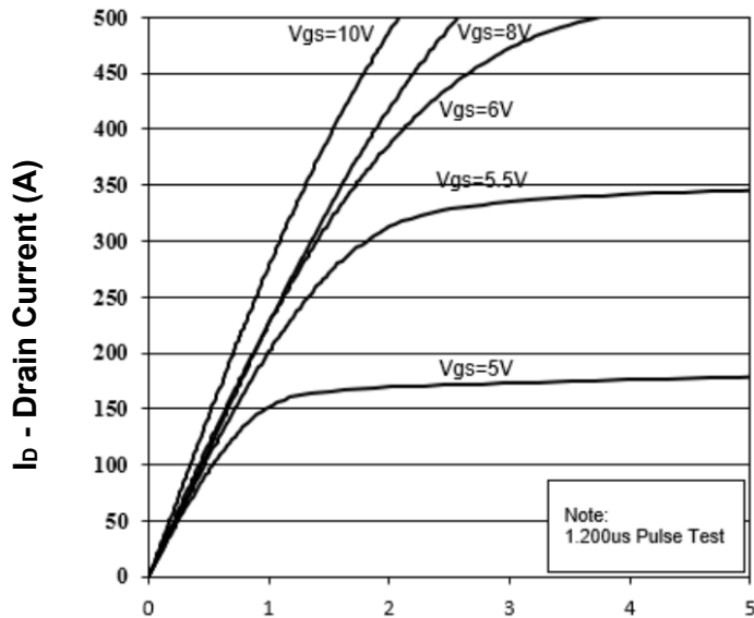
V_{DS} - Drain-Source Voltage (V)
