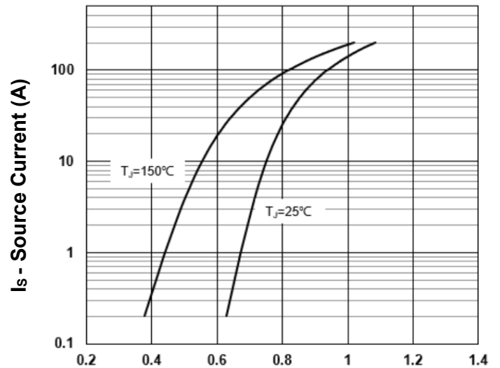
Diode Forward Current
