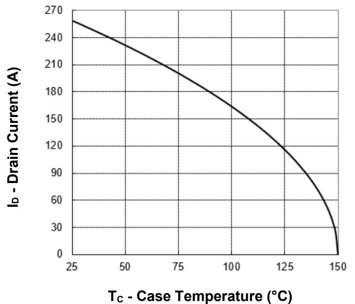
Current Capability
