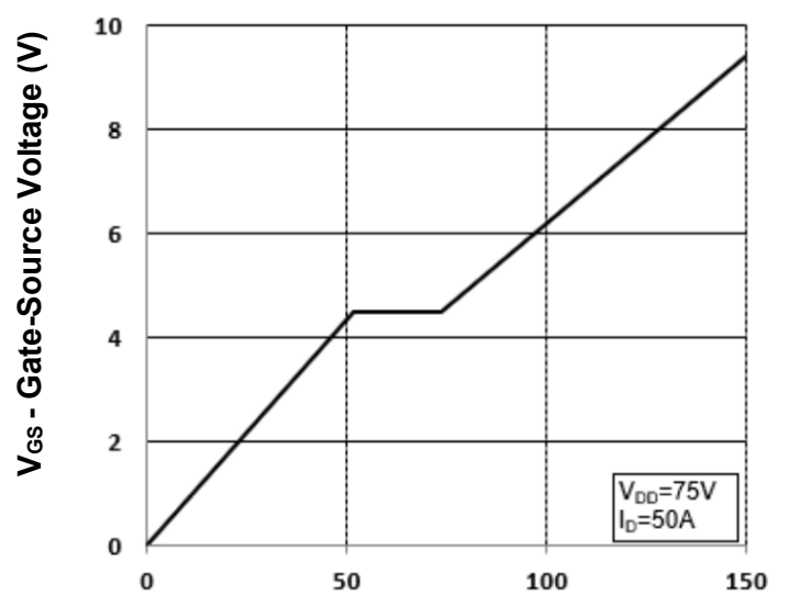
Gate Charge
